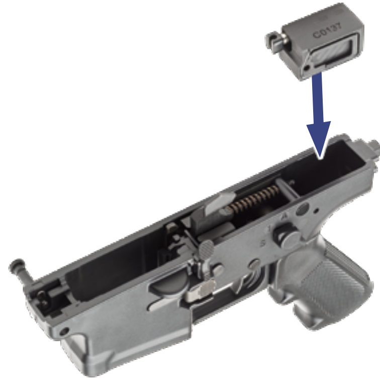
▶ FN SmartCore® integrated in the trigger module of an FN SCAR® rifle
